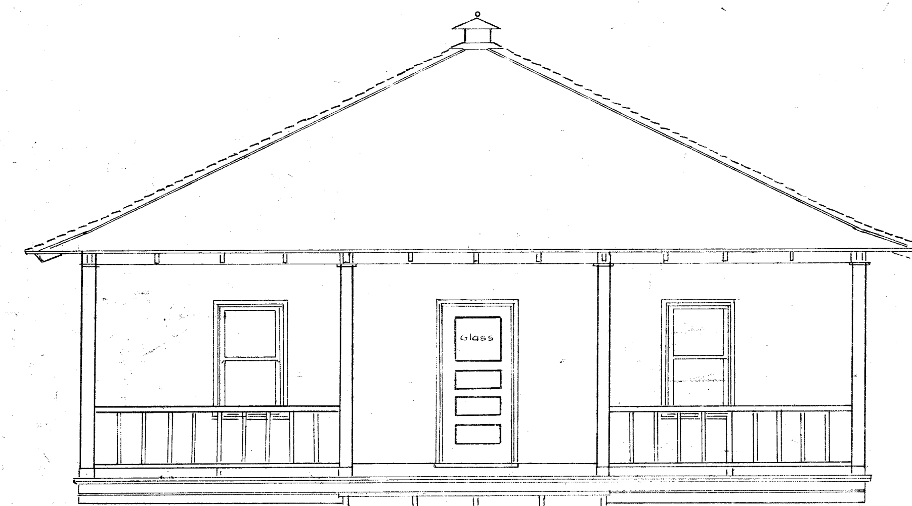
- Front -
