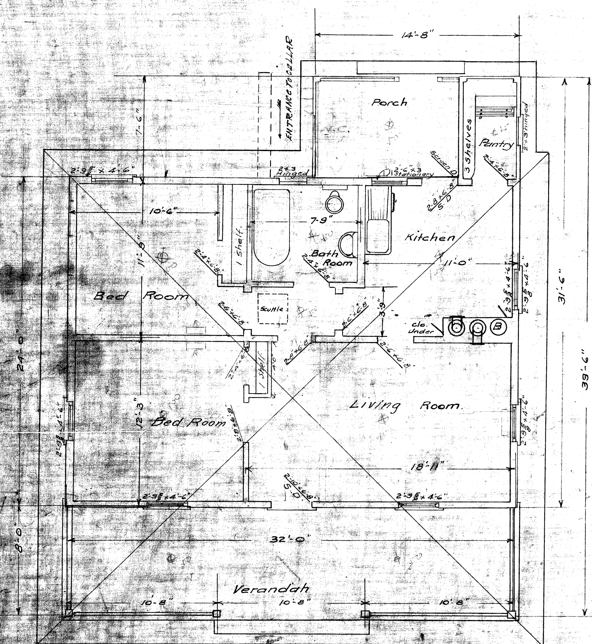
- Plan -
