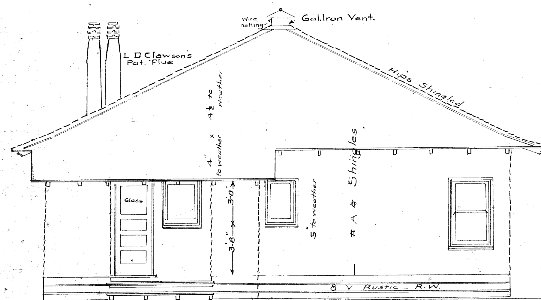
- Rear -
